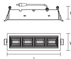
4 Cell Version
